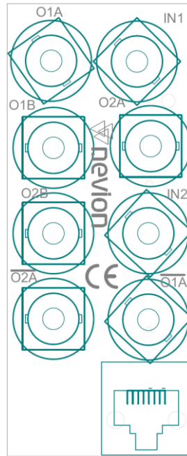
Figure 7: Overview of the DA-3GHD-2x4-C3 connector module
