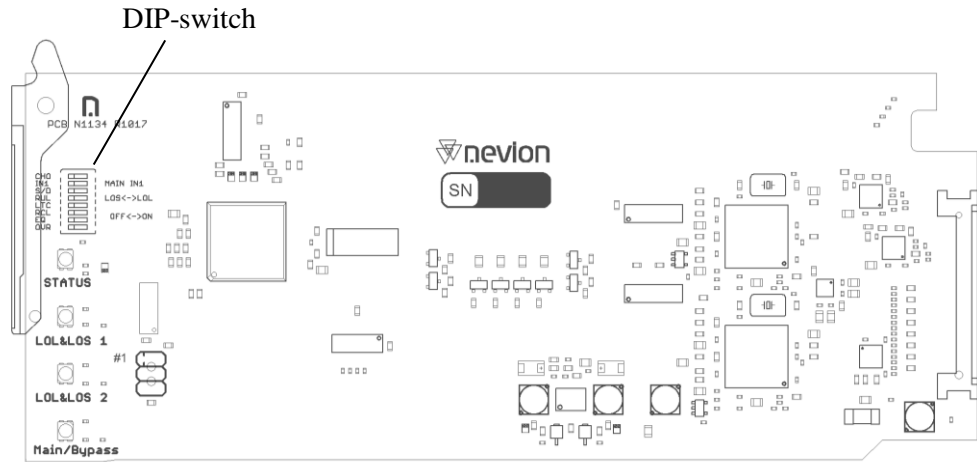
Figure 2: DA-3GHD-2x4 module DIP switches
