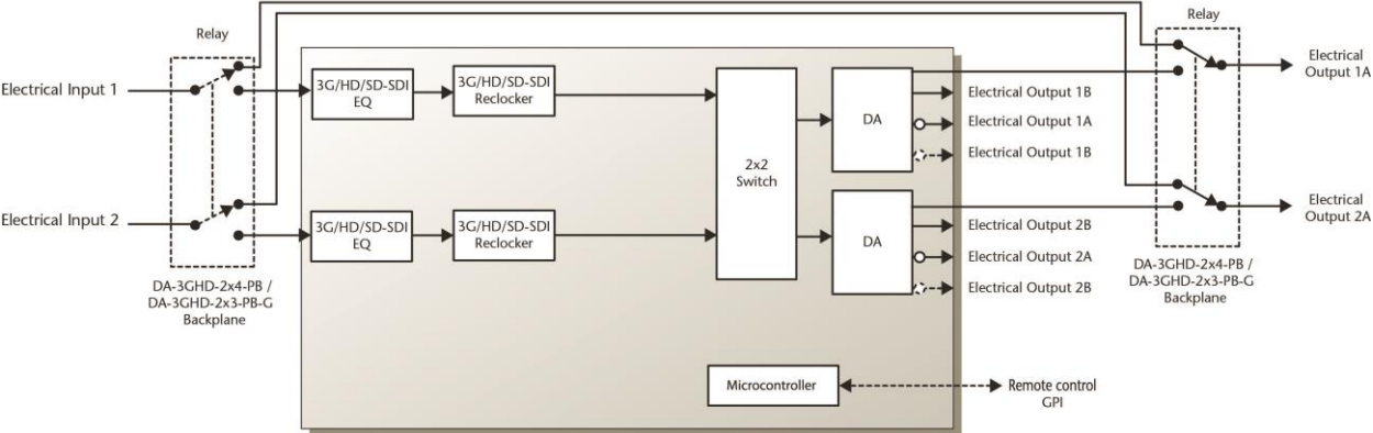
Figure 1: DA-3GHD-2x4 block diagram
