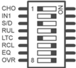
Figure 3: Distribution mode, Input 1 priority, Input 1 to all outputs, reclocker and equalizer on
