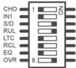
Figure 4: Distribution mode, Input 2 priority, Input 1 to 4 outputs, Input 2 to 4 outputs, transparent mode without equalization and reclocking.
